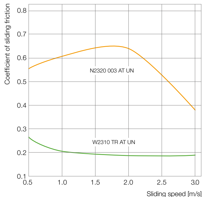
Fig. 10: Coefficient of sliding friction of Ultraform® N2320 003 AT and W2310 TR AT as a function of the sliding speed. Sample technically dry. Sliding counterpart: steel 100Cr6, HRc ca. 60, max. 67 °C, p = 4 \text{ MPa}
