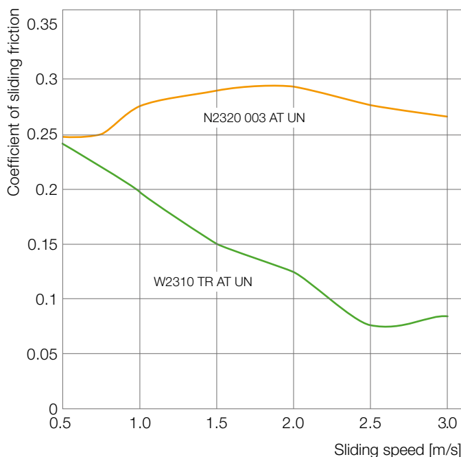
Fig. 9: Coefficient of sliding friction of Ultraform® N2320 003 AT and W2310 TR AT as a function of the sliding speed. Sample technically dry. Sliding counterpart: Ultraform® N2320 003 AT UN, max. 57 °C, p = 0.125 \text{ MPa}
